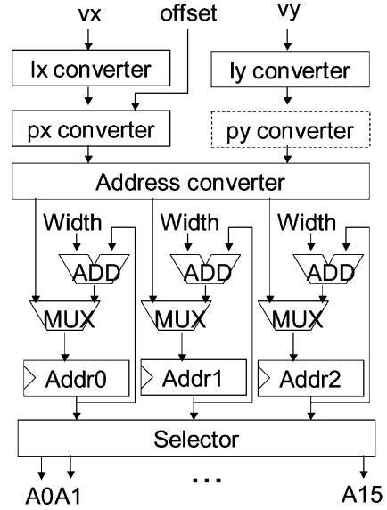
Fig. 15. Address generator.
