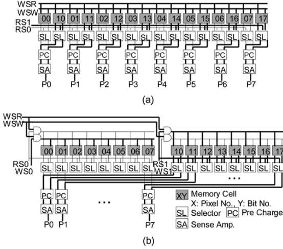
Fig. 16. Write-disturb-free memory cell arrangement. (a) Conventional method. (b) Proposed method.
