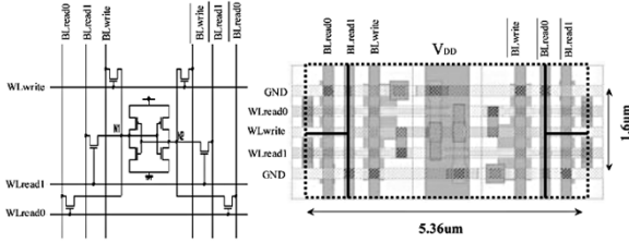
Fig. 17. Symmetric memory cell layout.
