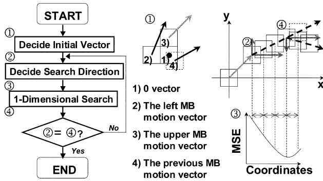
Fig. 1. GDS algorithm.
