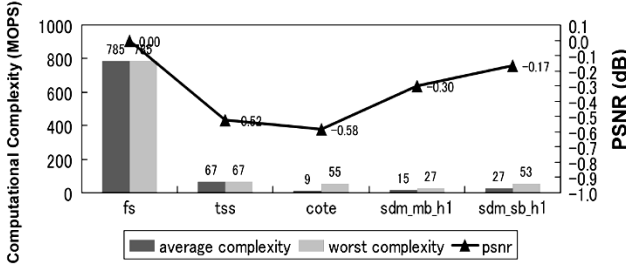
Fig. 5. ME algorithms comparison (QCIF 15 f/s).
