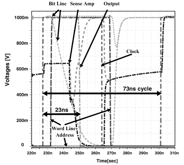
Fig. 19. Three-port SRAM simulation waveform.
