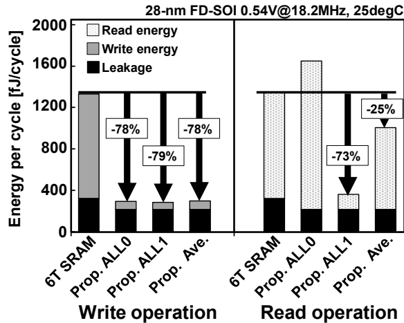
Fig. 10. Measured write energies, read energies, and comparison.
