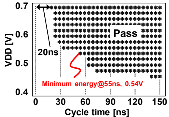
Fig. 9. Shmoo plot.
