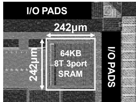
Fig. 8. Chip photo.
