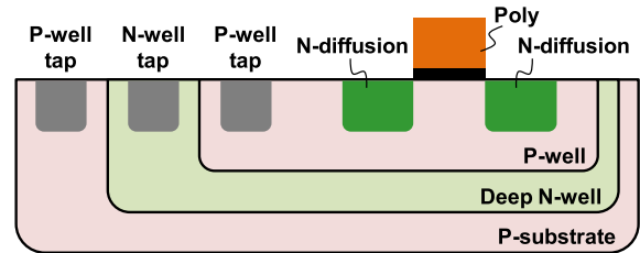
Fig. 7 Cross section of NMOS when using triple well.
