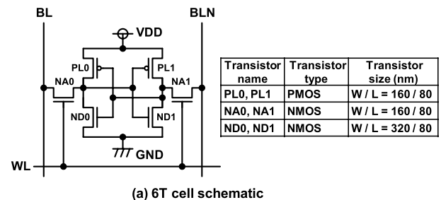
(a) 6T cell schematic
