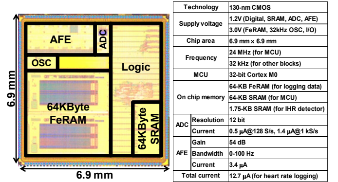
Figure 8. Chip photograph and chip specifications.
