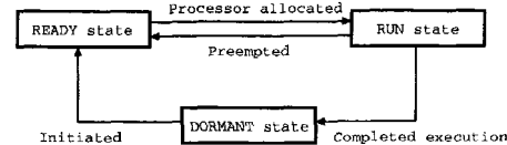
Figure 4. Task state transition.
