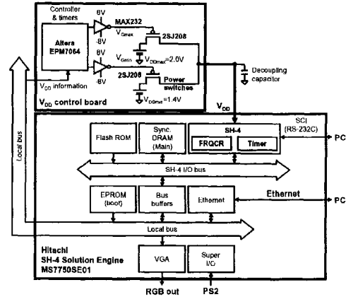
Figure 6. A block diagram of the hardware platform.
