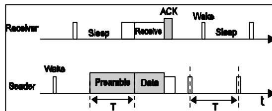
(a) Low Power Listening
