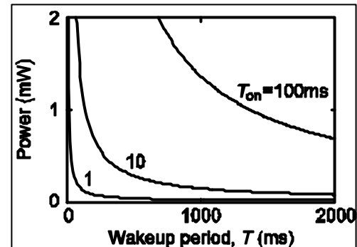
Figure 2. Relation of T to the idle power ( T_{on} = 1, 10 and 100 ms)
