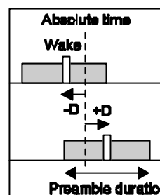
Figure 4. Maximum relative clock drift between nodes and preamble length
