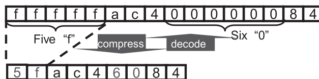
Fig. 6 Run Length Encoding (RLE) for GMM parameters.
