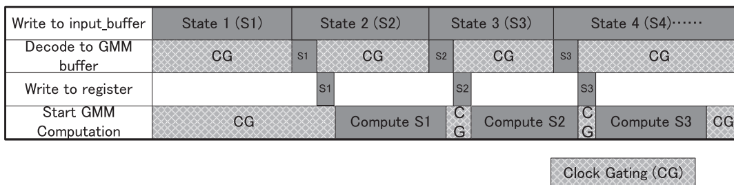
Fig. 5 Pipeline operation in GMM core.
