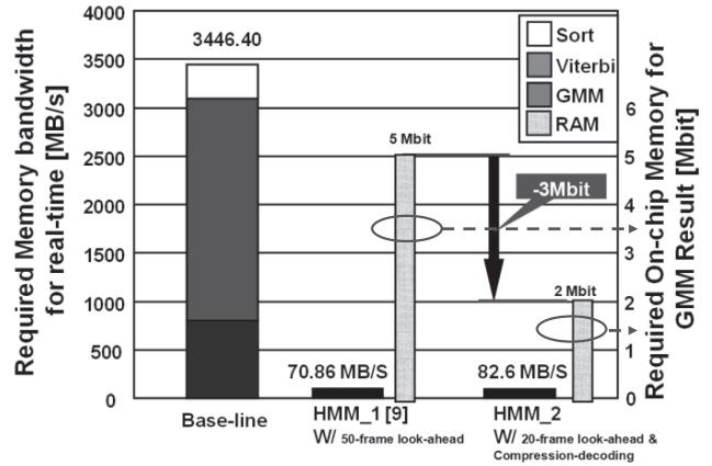
Fig. 15 Required memory bandwidth reduction & GMM result RAM reduction.
