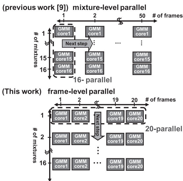
Fig. 8 20-frame parallel processing vs 16-mixture parallel processing.
